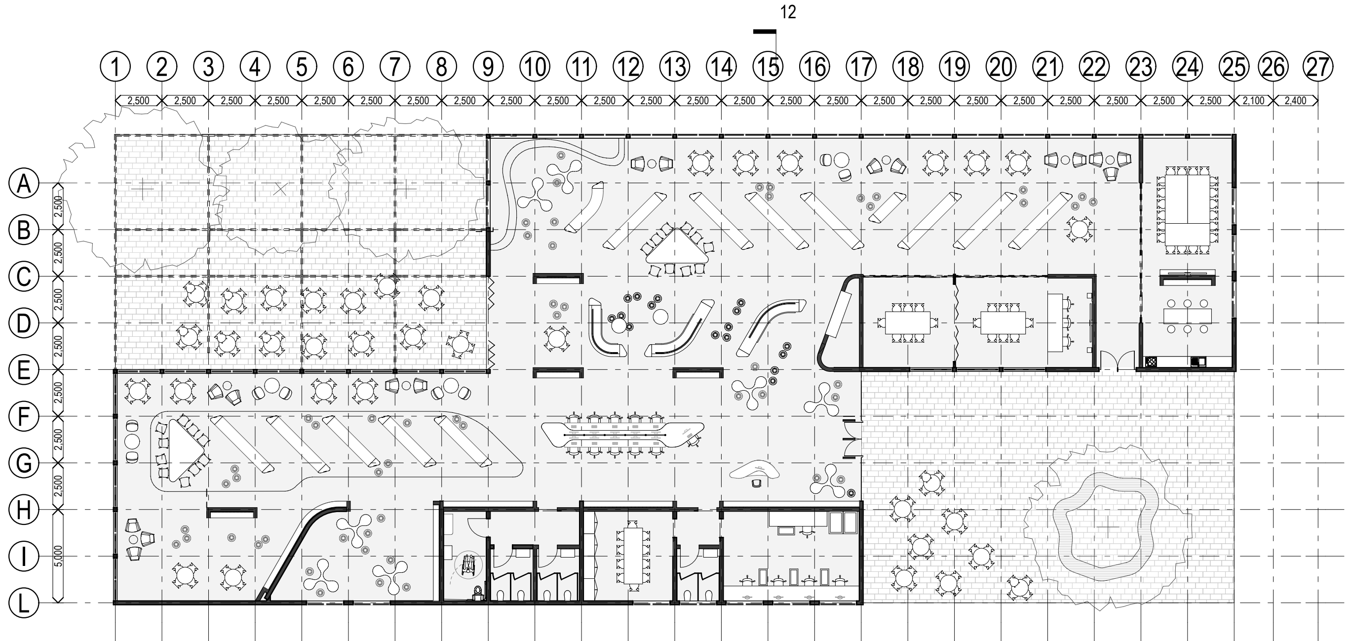
1000 msq Library Plan 1:200
