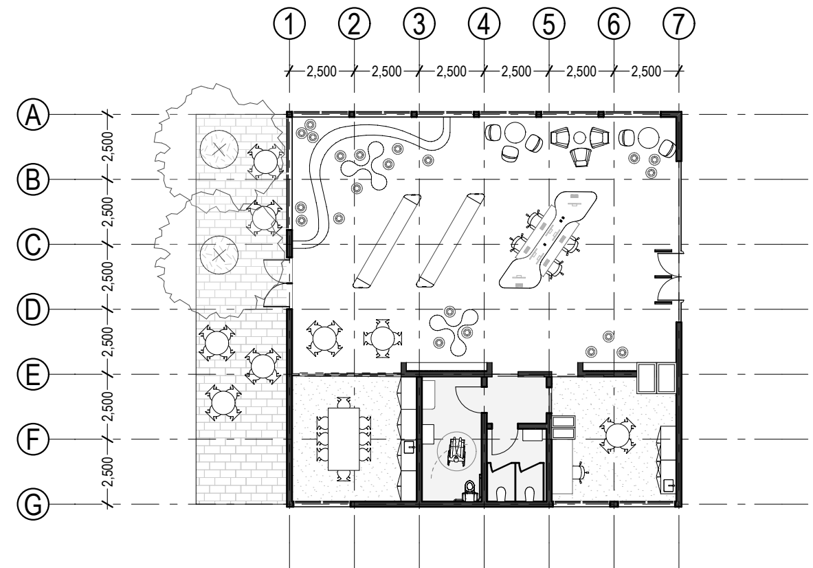
190 msq Library Plan 1:200
