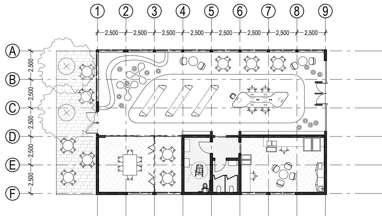
250 msq Library Plan 1:200
