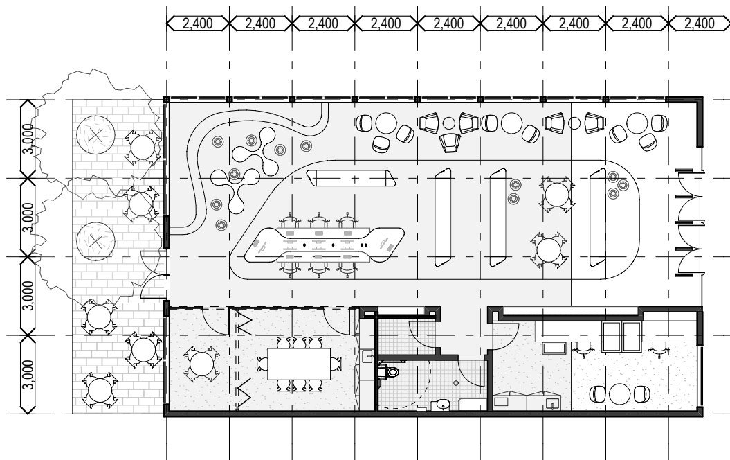
250sqm Library 1:200
