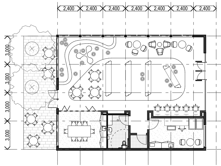
190 sqm library 1:200
